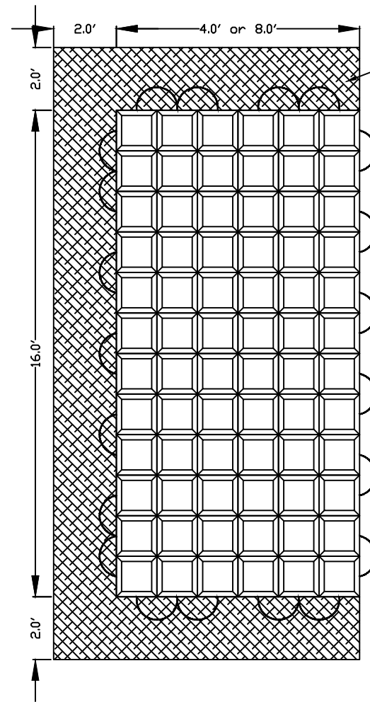
2 CC-70 MATTRESS W/ GEOTEXTILE NOT TO SCALE
