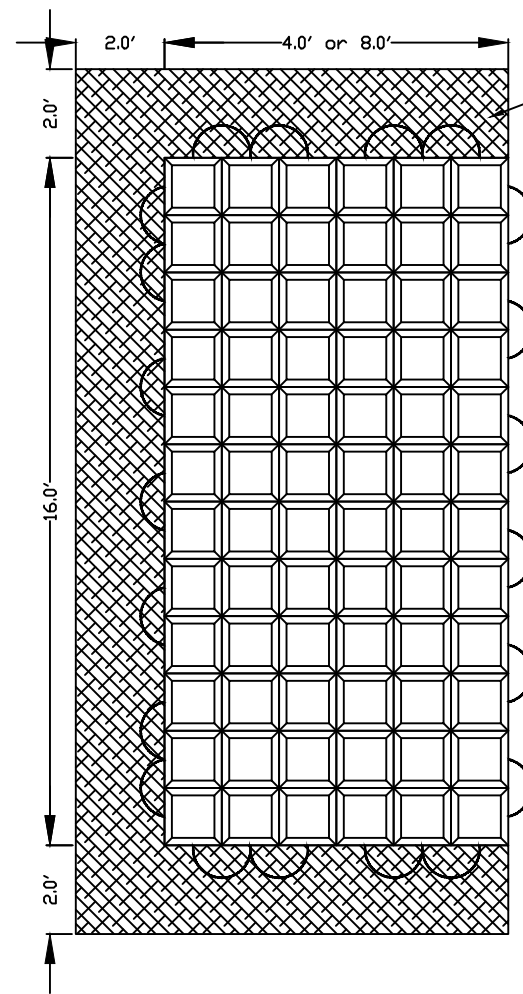
2 CC-20 MATTRESS W/ GEOTEXTILE NOT TO SCALE
